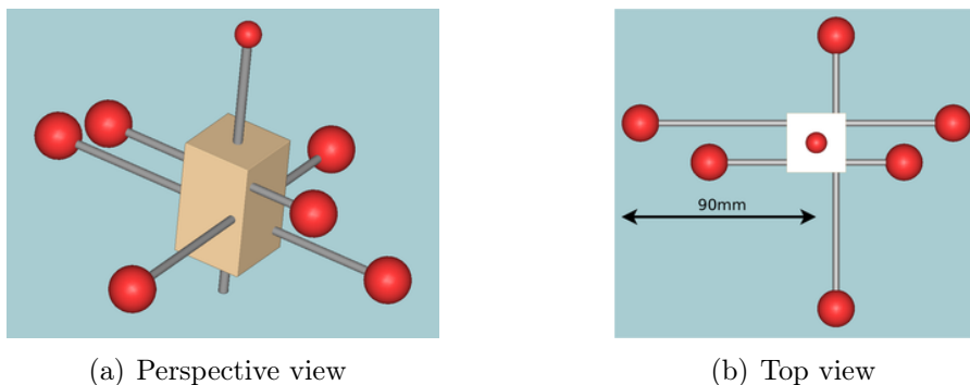
Figure 6: RoCKIn Marker Set used during the RoCKIn 2014 Competition (the motion capture markers are illustrated as red spheres)
