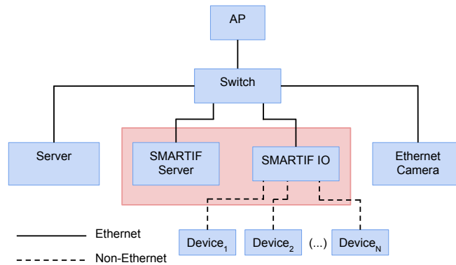
Figure 5: Network infrastructure of the RoCKIn@Home Competition
